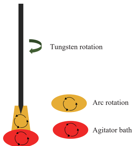
Fig. 1 Schematic diagram of RT-GTAW
